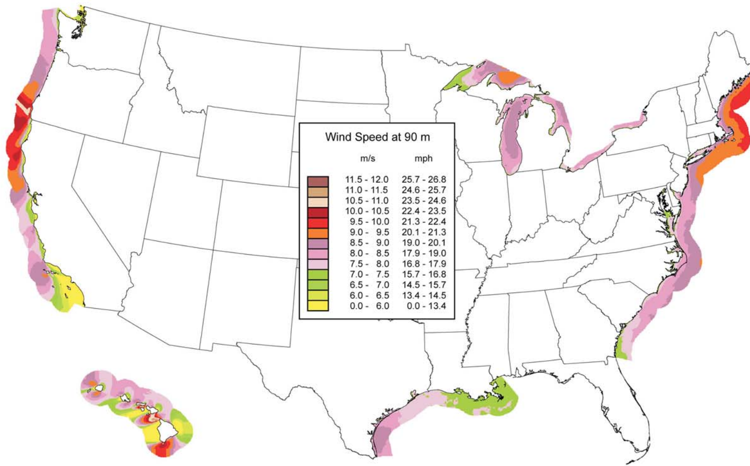
Figure 4.14 Offshore Wind Resources
